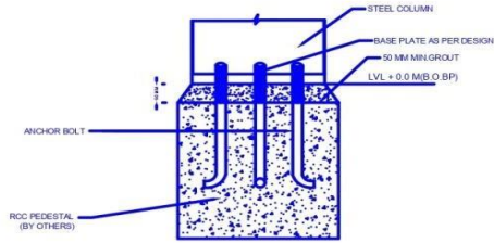
SAMPLE DETAILS OF MINIMUM PEDESTAL REQ FOR PINNED BASE FOR ALL LEAN TO COLUMN
