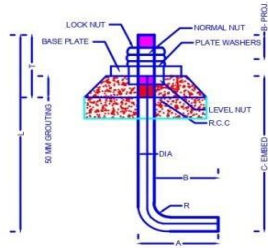
ANCHORED BOLT - @20
